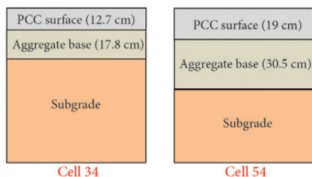
Fig. 1. Schematic cross-section of rigid pavement sections tested (not to scale)
