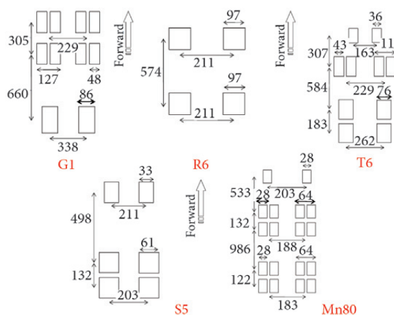
Fig. 2. Dimensions for test vehicles (dimension unit – cm; not to scale)
