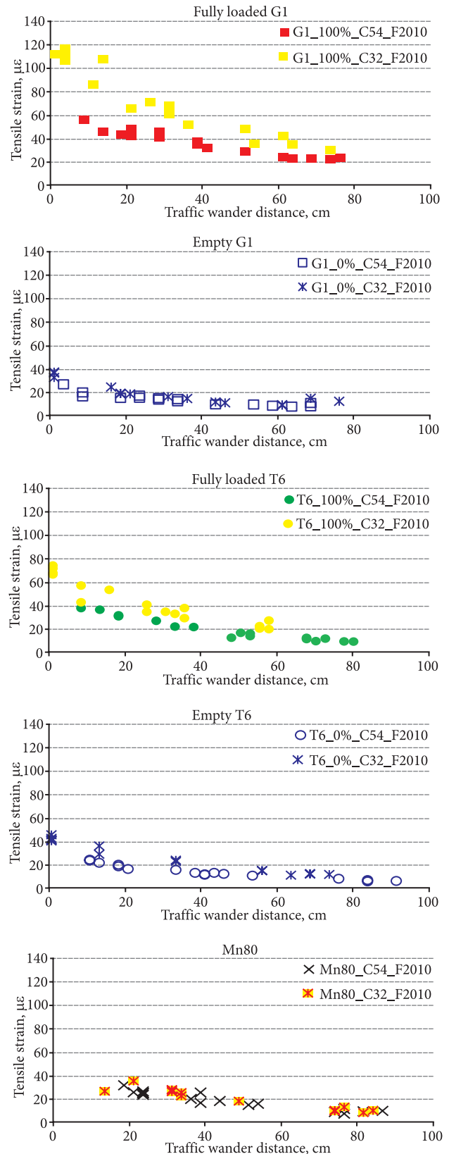
Fig. 9. Effect of PCC pavement structure on tensile strains at the bottom of the PCC slab near mid-slab edge
