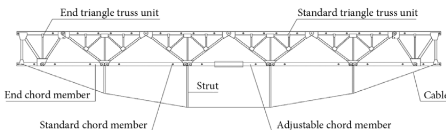
Fig. 1. Major components of the TSS (truss string structure)
