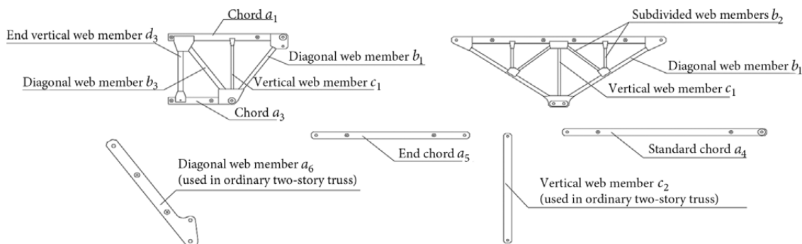
Fig. 2. Components of the assembly truss unit
